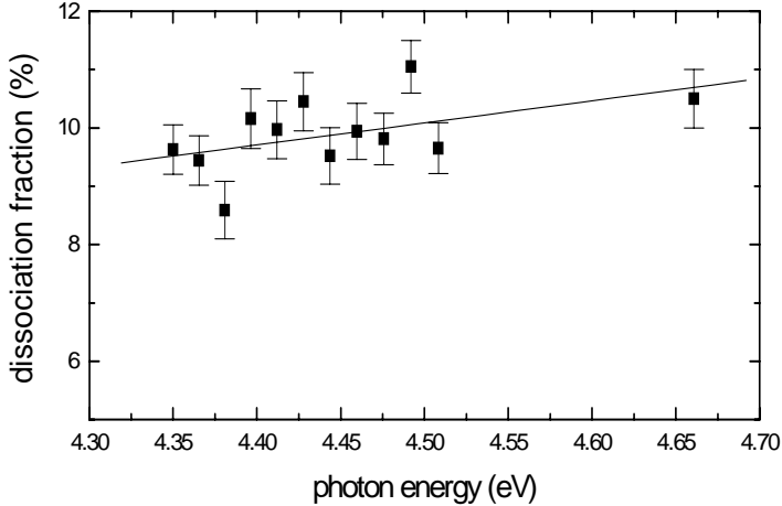
Figure 5.3: Fraction of dissociation versus excitation energy. The dissociation fraction is defined as number of O fragments versus total number of detected particles ( O and O_2 ).
